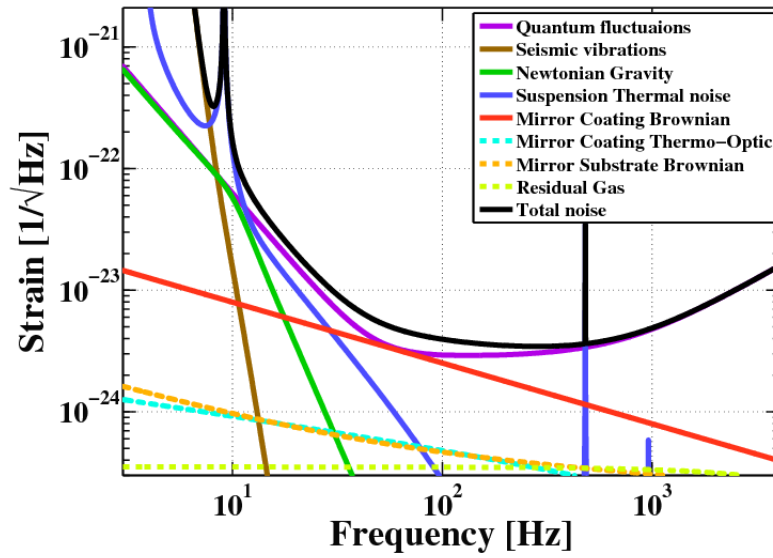
Figure 5: [20]Noise curve for advanced LIGO detectors.
